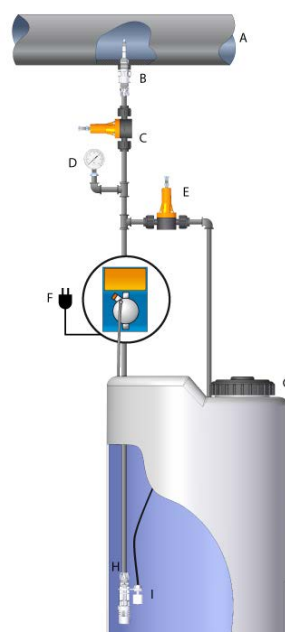
Fig. 6 - Installation type
